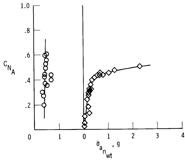
Figure 28. F-111 TACT aerodynamic summary for \bar{q} = 38.3 \text{ kN/m}^2 (800 lb/ft 2 ). M = 0.90 .
