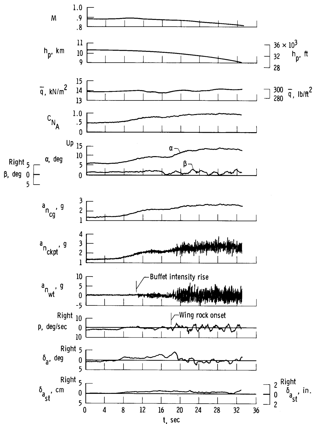
Figure 5. Time history of smooth windup turn illustrating flow separation at higher angles of attack. F-111 TACT airplane; \Lambda = 26^\circ .
