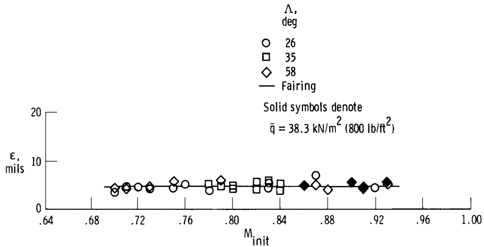
(a) F-111A airplane.
