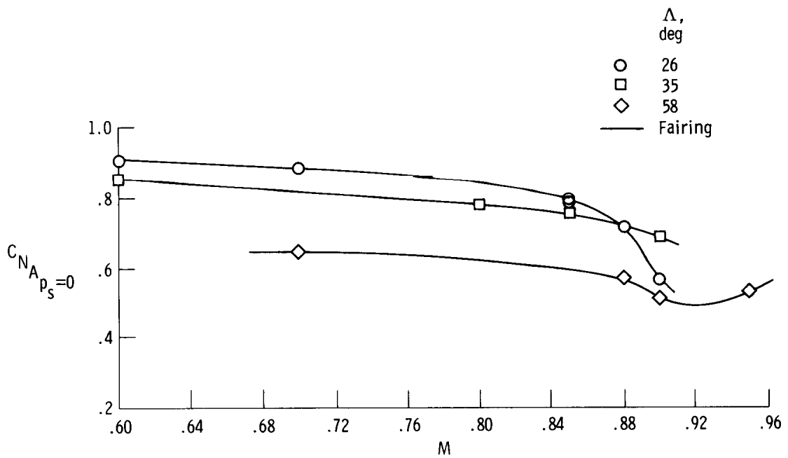
(b) F-111 TACT airplane.
