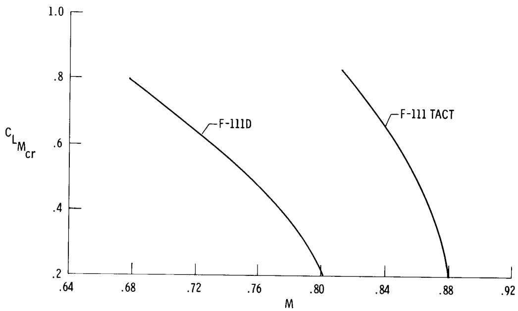
Figure 35. Comparison of drag-rise Mach numbers for F-111D and F-111 TACT models at \Lambda = 26^\circ (ref. 9).
