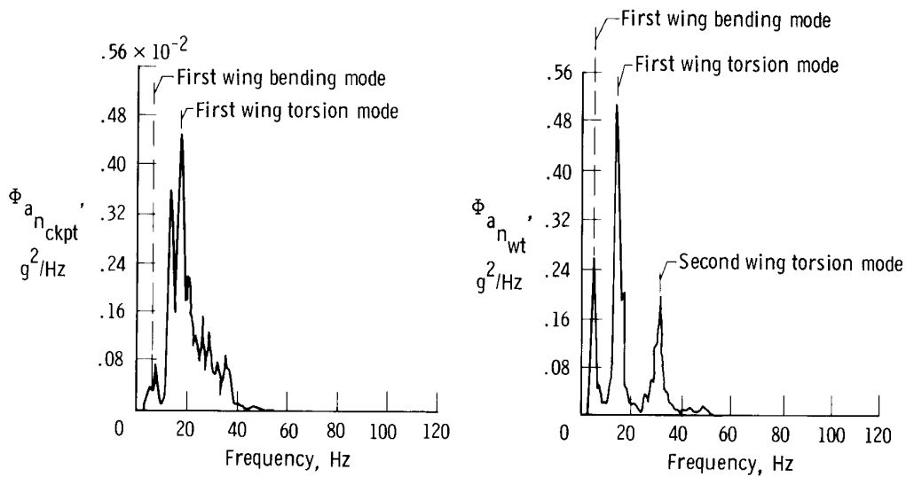
(a) M_{init} = 0.82 , \Lambda = 26^\circ , \alpha_{init} = 10^\circ .
