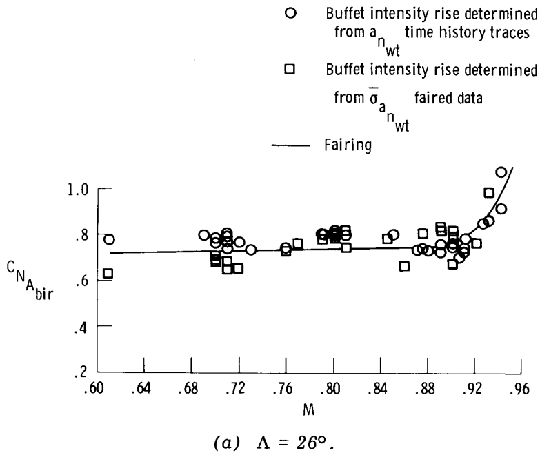
Figure 8. F-111 TACT buffet intensity rise boundaries.
