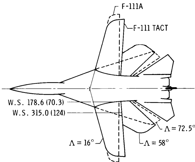
(a) Aircraft plan views.
