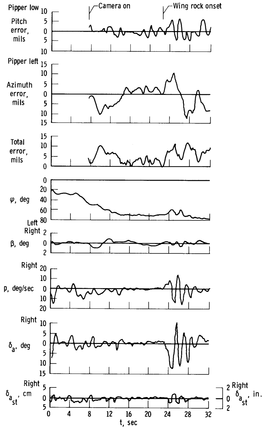
Figure 17. Time history of F-111 TACT tracking windup illustrating effects of adverse yaw and wing rock.
