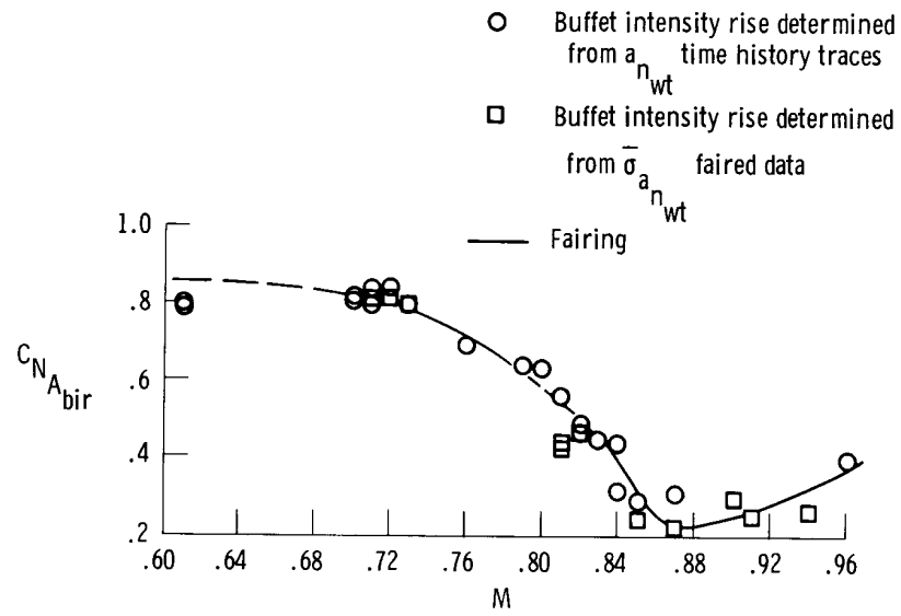
(a) \Lambda = 26^\circ .
