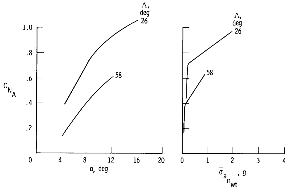
(b) F-111 TACT airplane.
