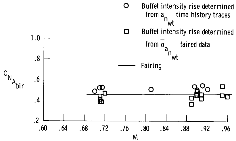
(c) \Lambda = 58^\circ .
