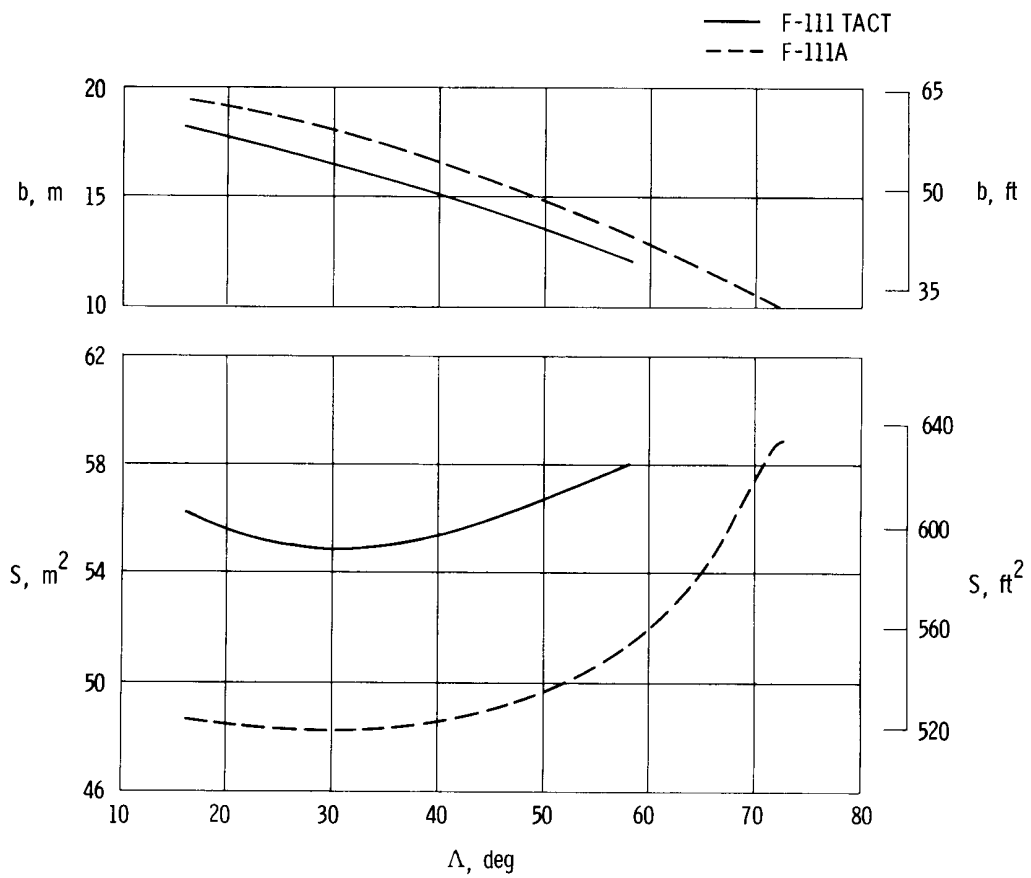
Figure 3. Changes in wing geometry and wing-sweep position for F-111A and F-111 TACT aircraft.
