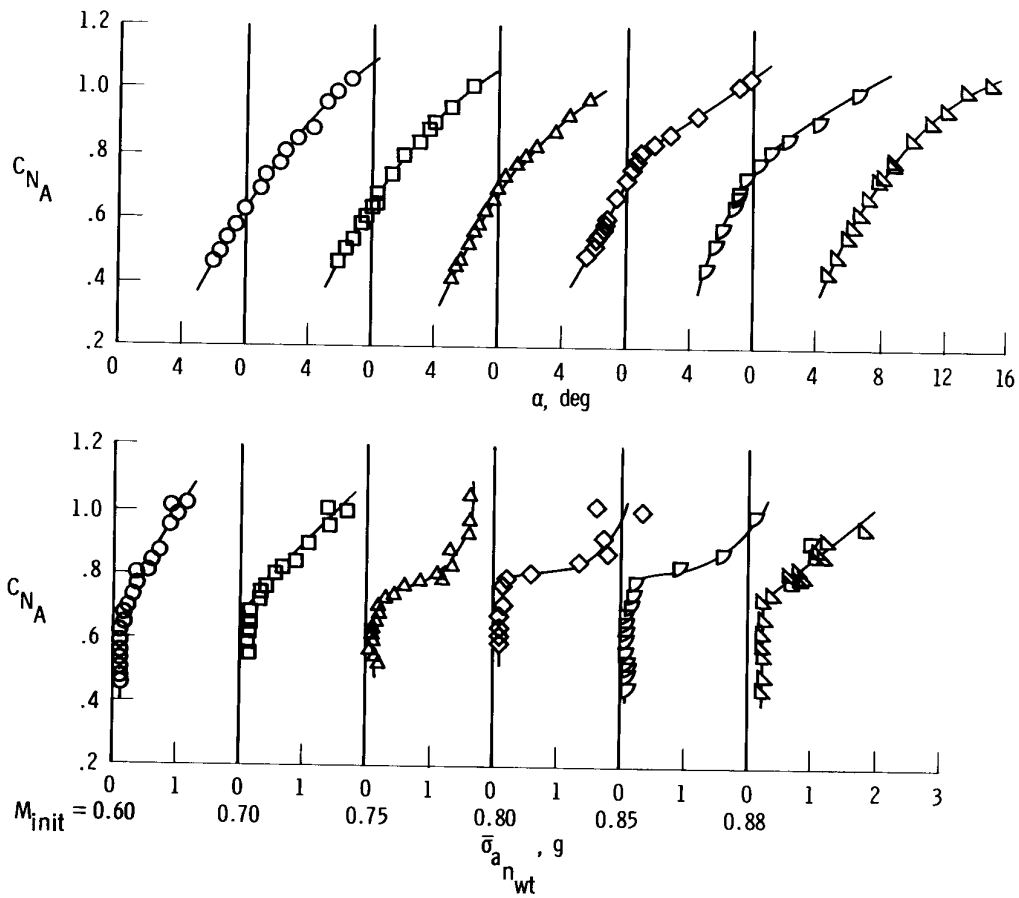
(a) \Lambda = 26^\circ .
