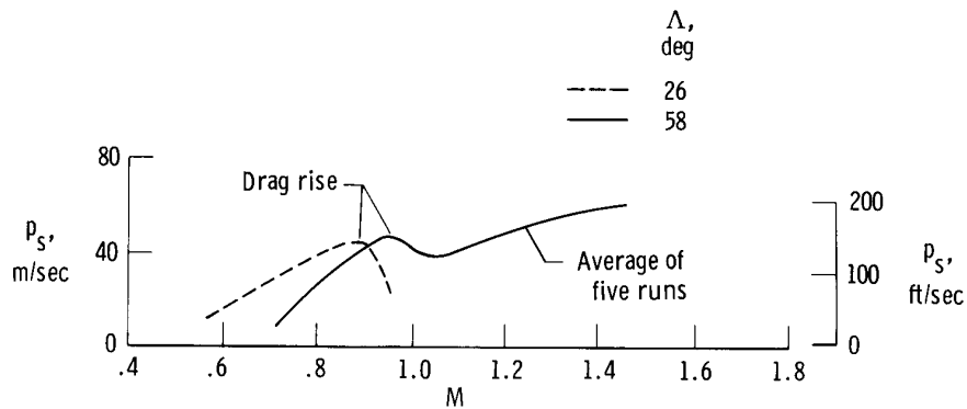
(b) F-111 TACT airplane. All data from this study.
