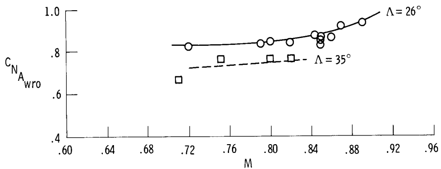
(b) F-111 TACT airplane.
