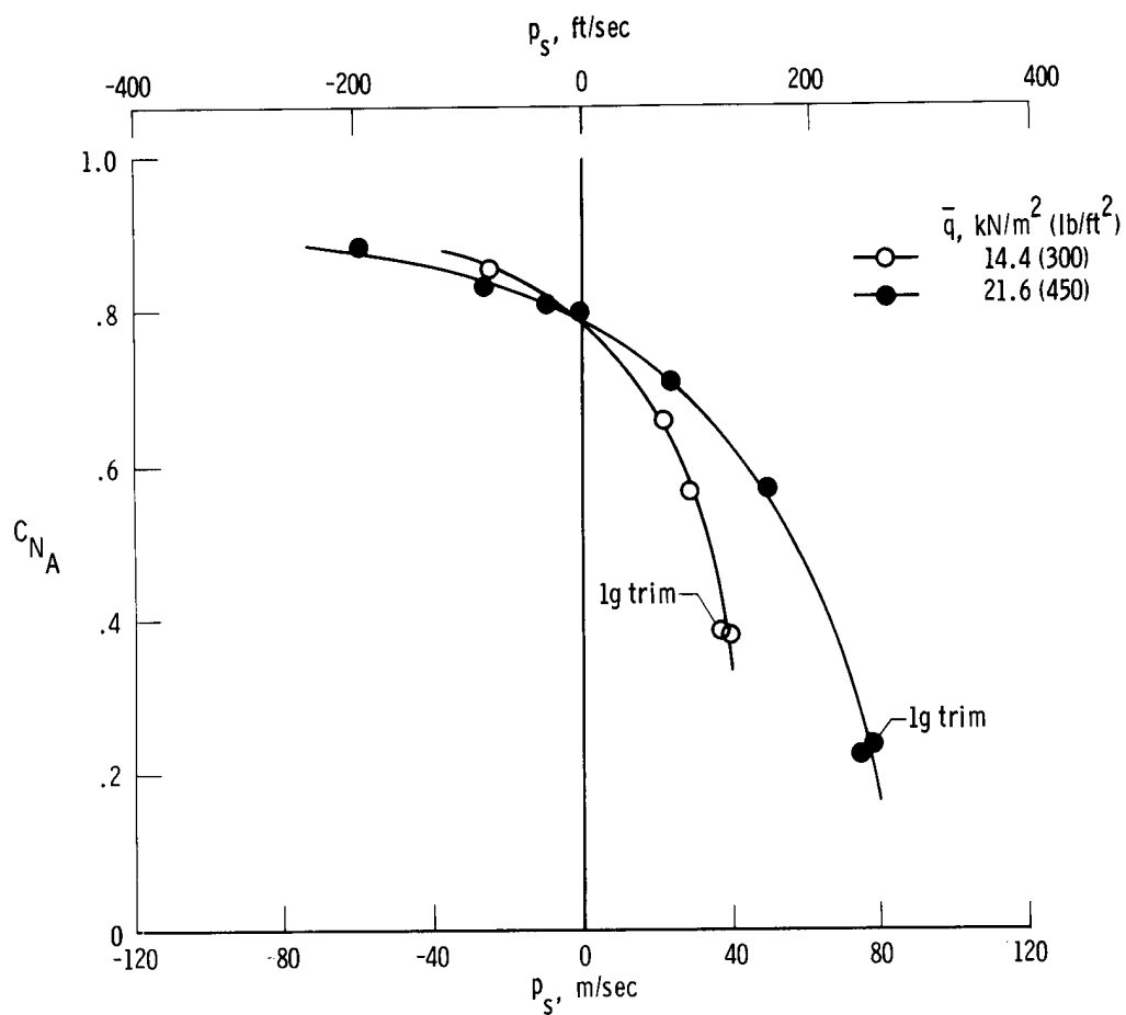
Figure 34. Dynamic pressure effect on specific excess power variation obtained on F-111 TACT airplane at M = 0.85 . \Lambda = 26^\circ .
