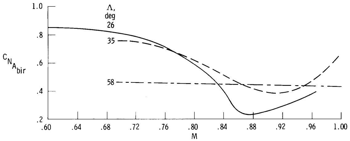
(a) F-111A airplane.
