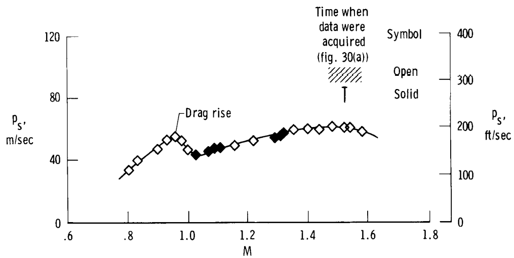
(b) 1g specific excess power variation.
