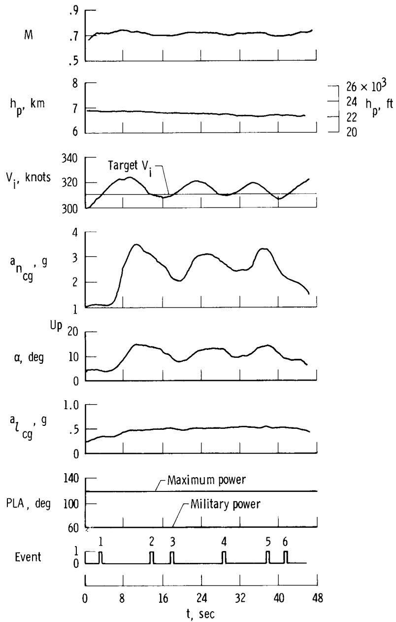
(a) Time history.
