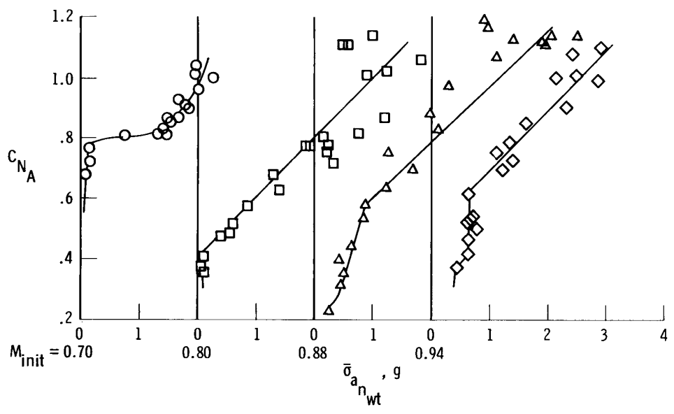
(a) \Lambda = 26^\circ .
