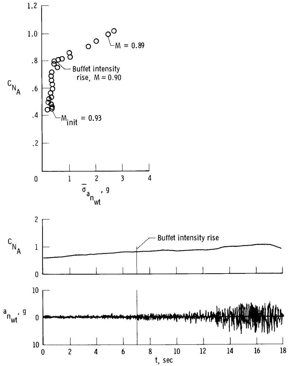
Figure 24. Buffet intensity rise determination.
