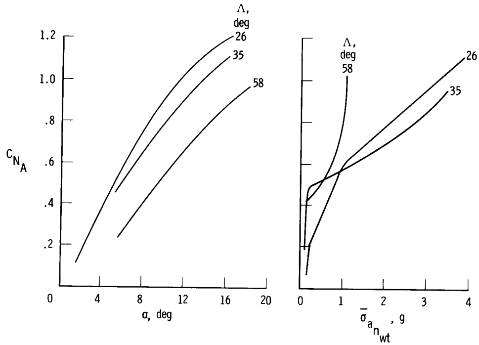
(a) F-111A airplane.
