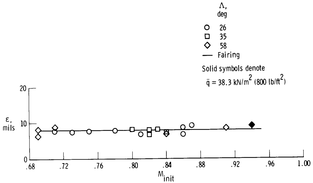
(a) F-111A airplane.
