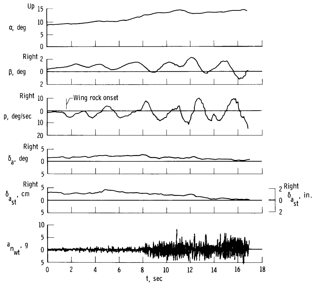
(b) Roll augmentation off.
