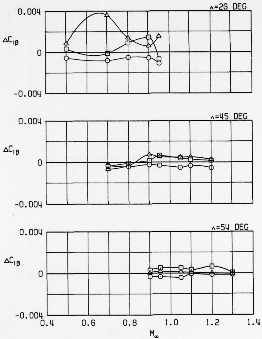
c. Four GBU-15CCW stores Figure 17. Continued.
