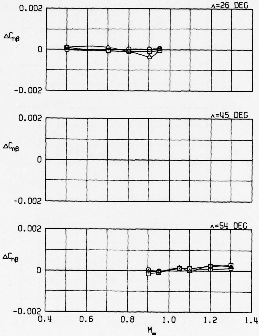
Figure 16. Effects of external stores on the static directional stability derivative.
