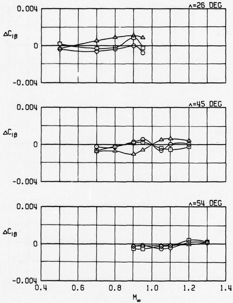
g. 12 Rockeye stores (outboard pylons) Figure 17. Continued.
