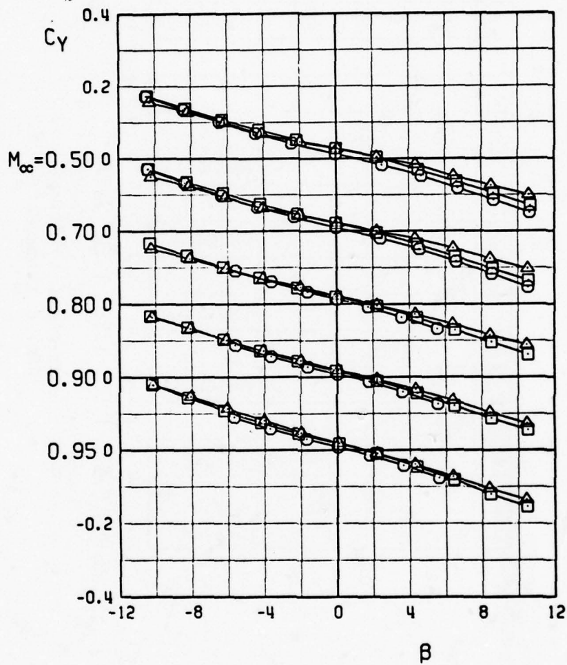
d. Side-force coefficient, \Lambda = 26 deg Figure 8. Continued.
