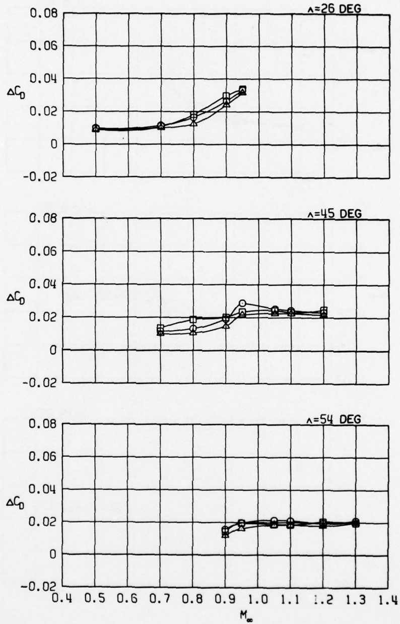
b. Four GBU-10 stores Figure 15. Continued.
