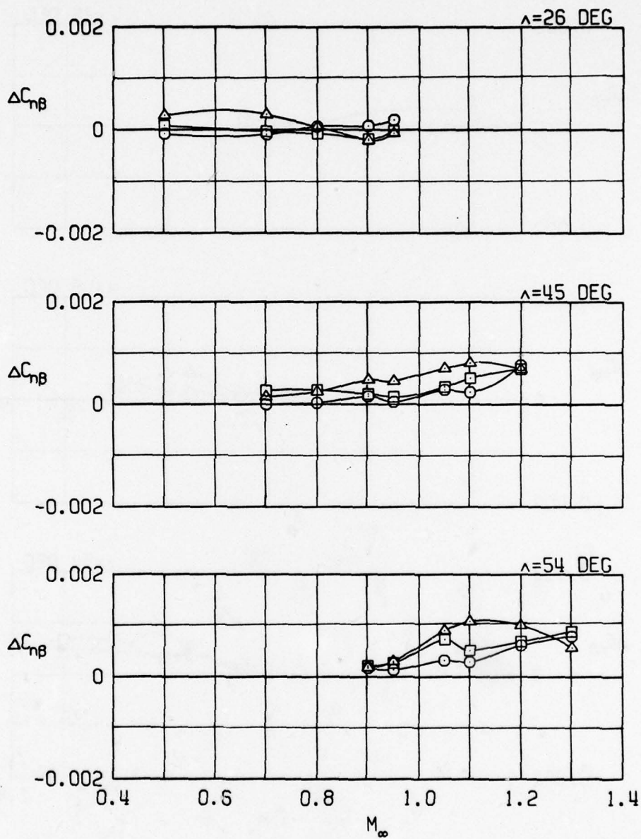
h. 12 SUU-30 stores (outboard pylons) Figure 16. Continued.
