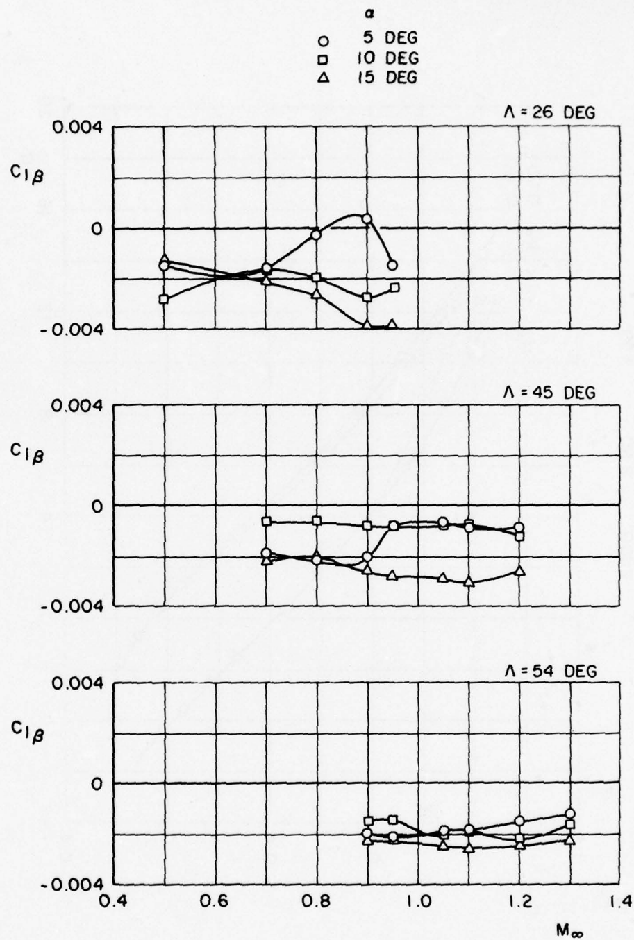
e. Effective dihedral Figure 9. Concluded.
