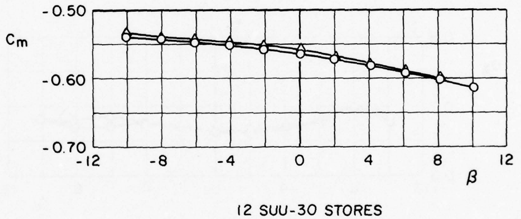
b. Pitching-moment coefficient Figure 13. Continued.
