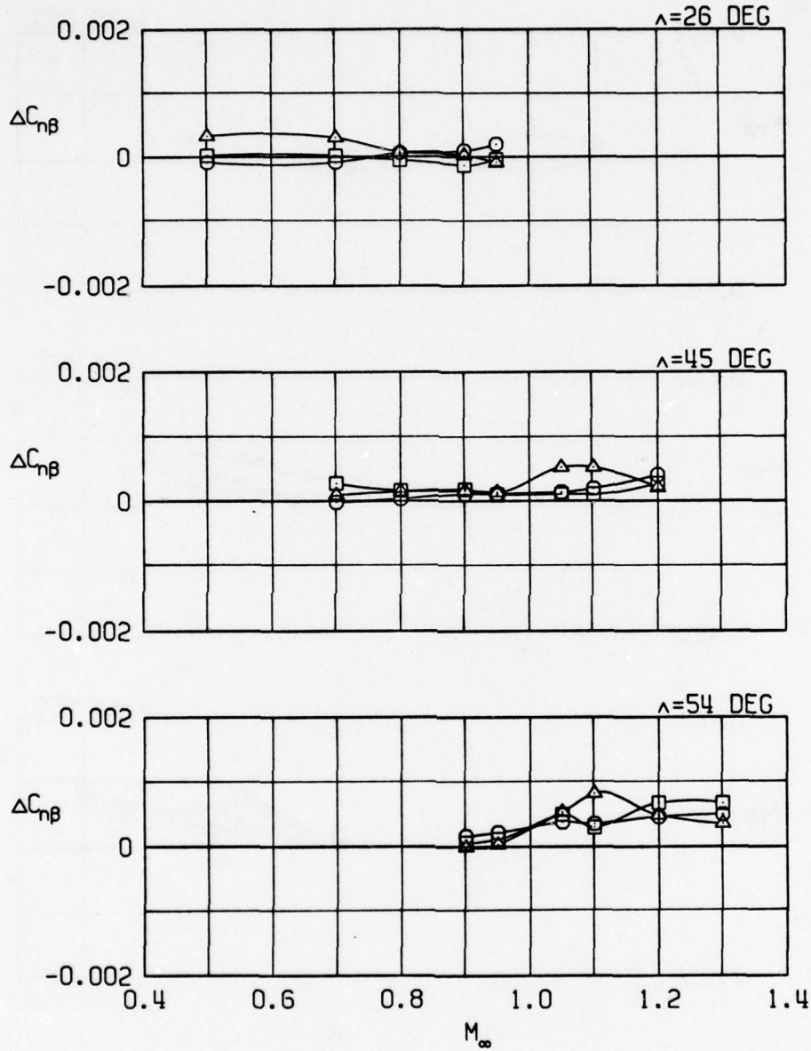
i. 12 MK-82SE stores (outboard pylons) Figure 16. Continued.
