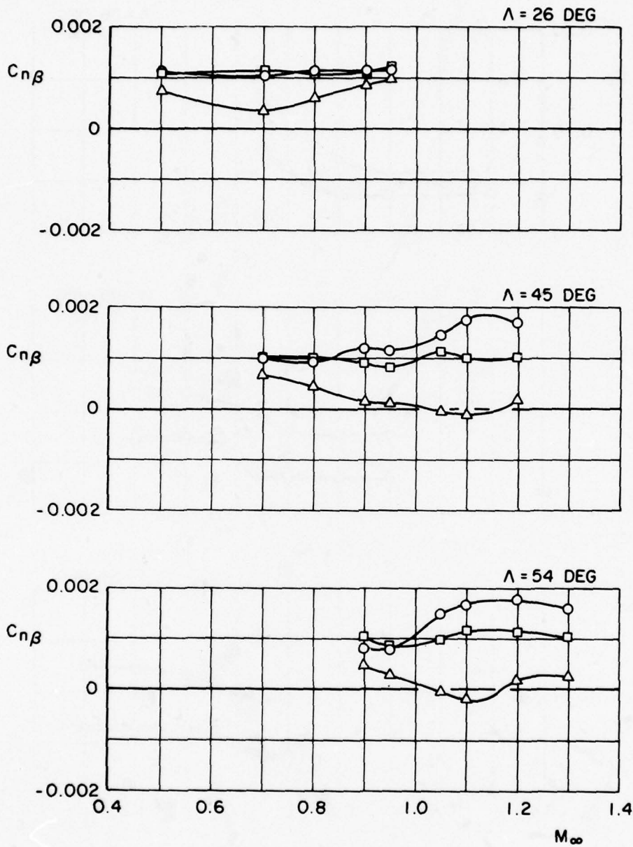
d. Static directional stability derivative Figure 9. Continued.
