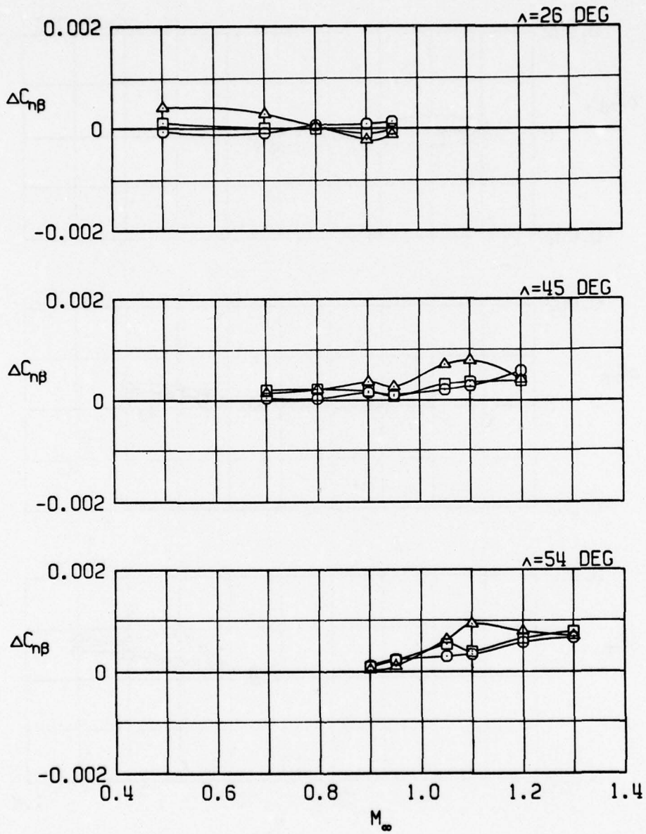
g. 12 Rockeye stores (outboard pylons) Figure 16. Continued.
