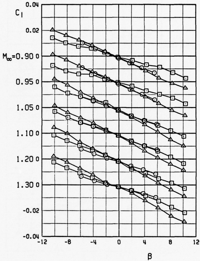
f. Concluded, \Lambda = 54 deg Figure 8. Concluded.
