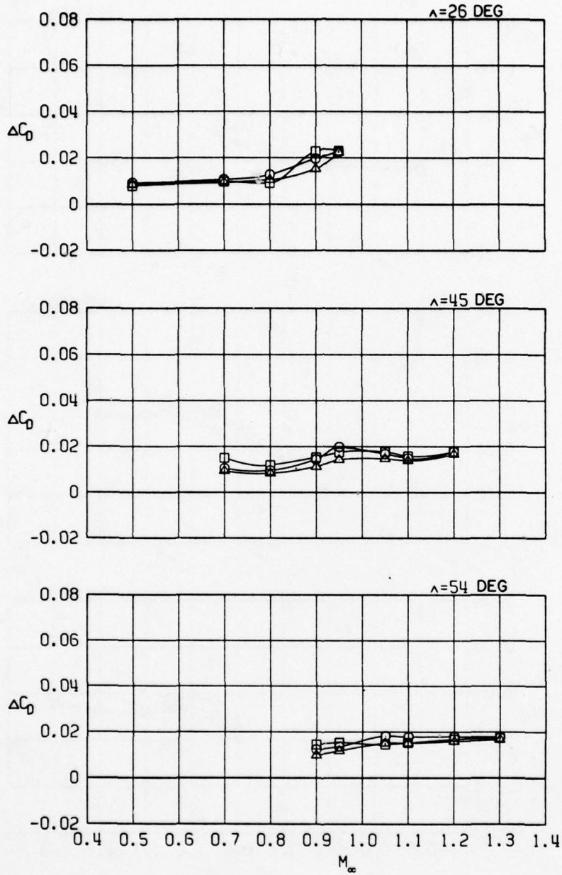
i. 12 MK-82SE stores (outboard pylons) Figure 15. Continued.
