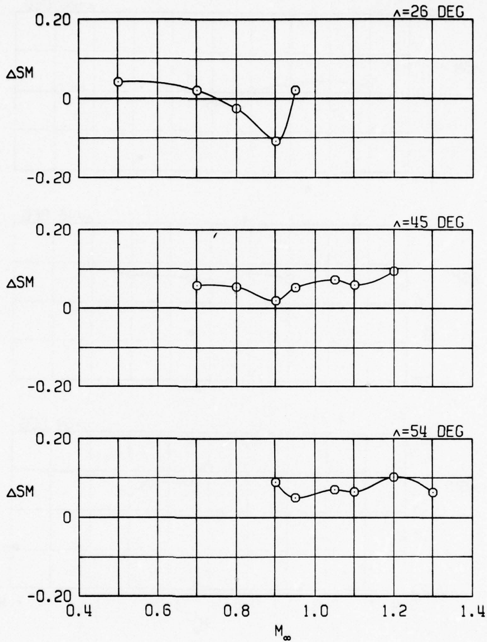
b. Four GBU-10 stores Figure 14. Continued.
