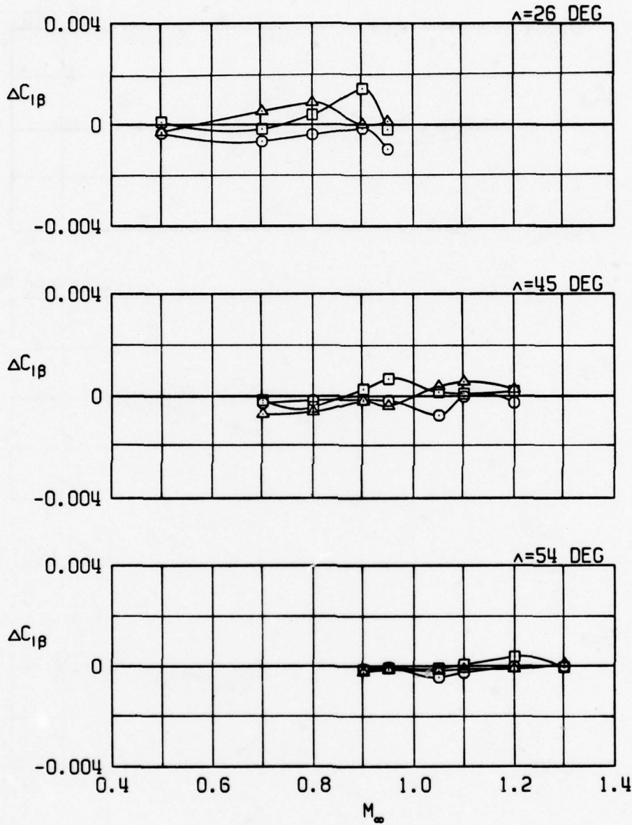
i. 12 MK-82SE stores (outboard pylons) Figure 17. Continued.
