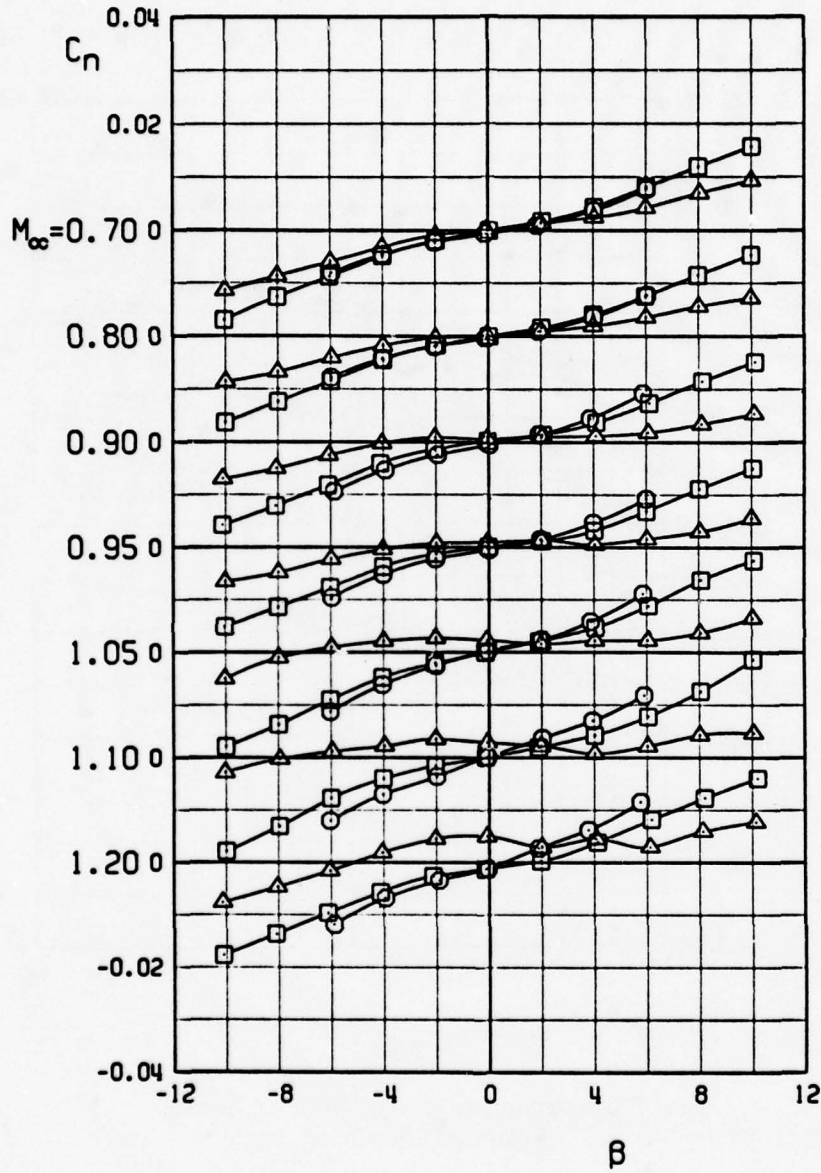
e. Continued, \Lambda = 45 deg Figure 8. Continued.
