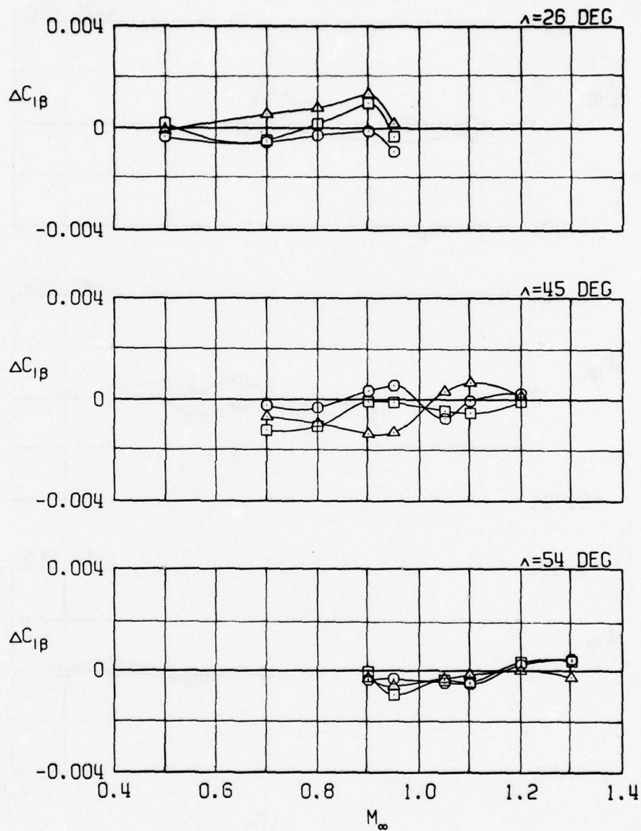
h. 12 SUU-30 stores (outboard pylons) Figure 17. Continued.
