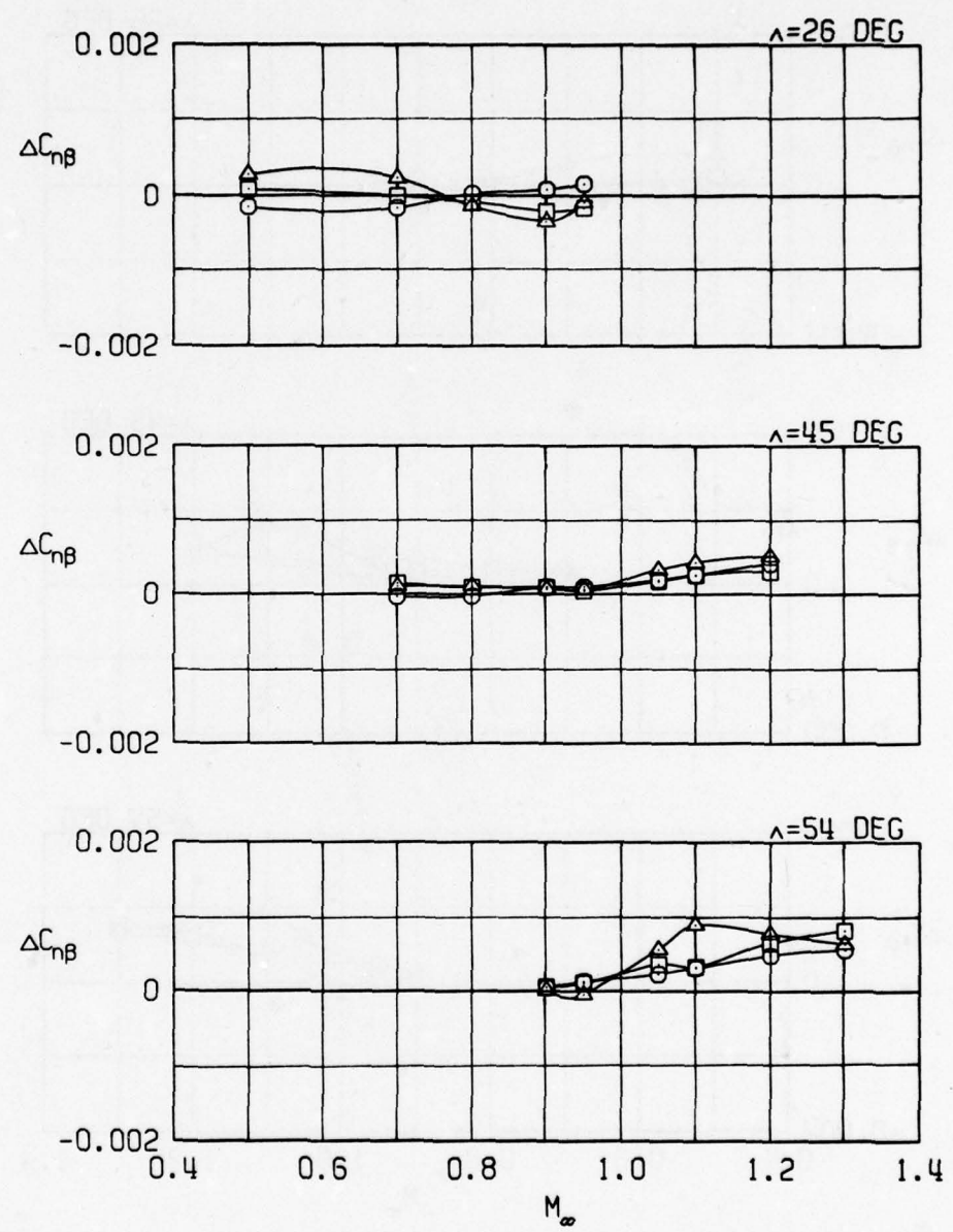
f. 16 Rockeye stores (slant 4 loading) Figure 16. Continued.
