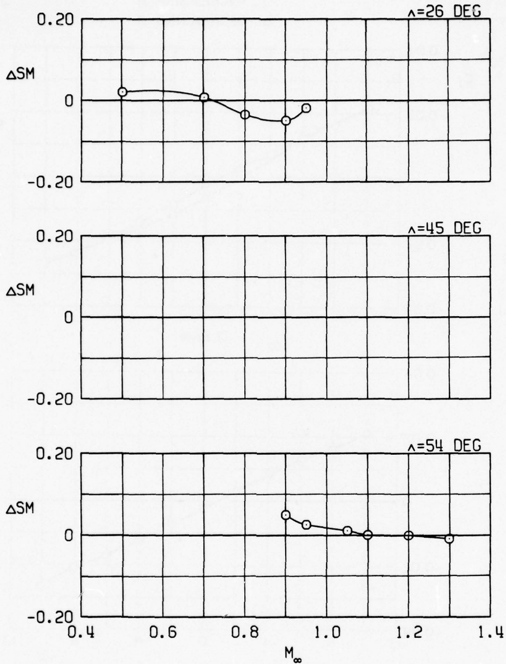
a. Pylons alone Figure 14. Effects of external stores on the static margin.
