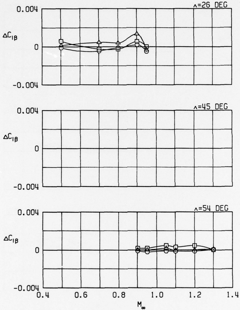
a. Pylons alone Figure 17. Effects of external stores on the effective dihedral.
