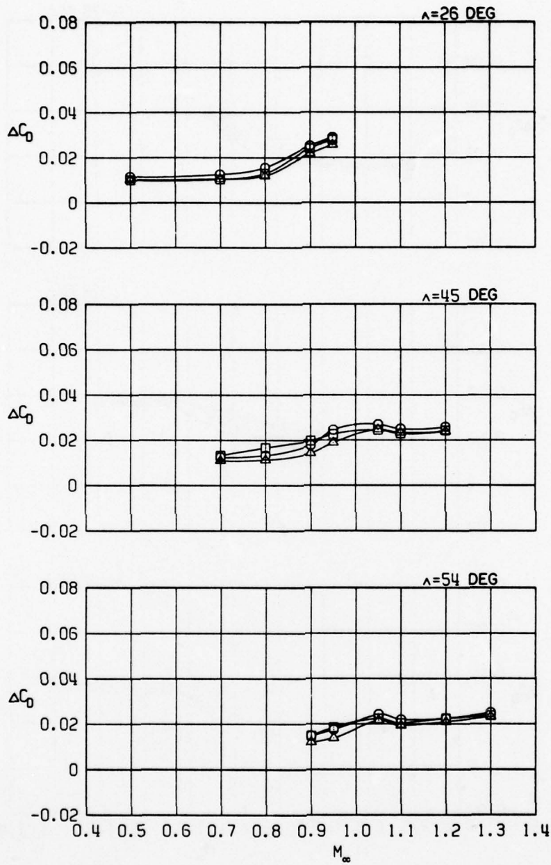
g. 12 Rockeye stores (outboard pylons) Figure 15. Continued.
