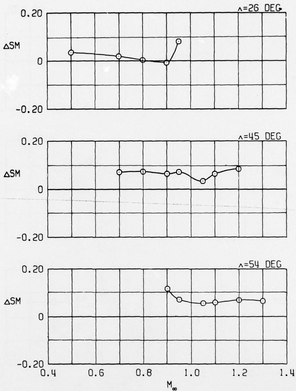
h. 12 SUU-30 stores (outboard pylons) Figure 14. Continued.
