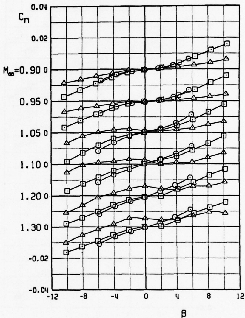
e. Concluded, \Lambda = 54 deg Figure 8. Continued.
