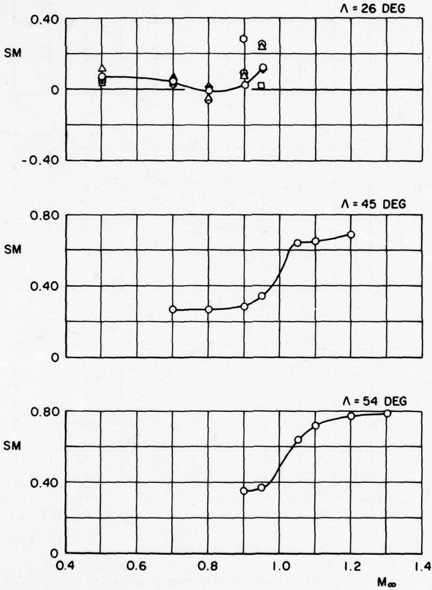
b. Static margin Figure 9. Continued.
