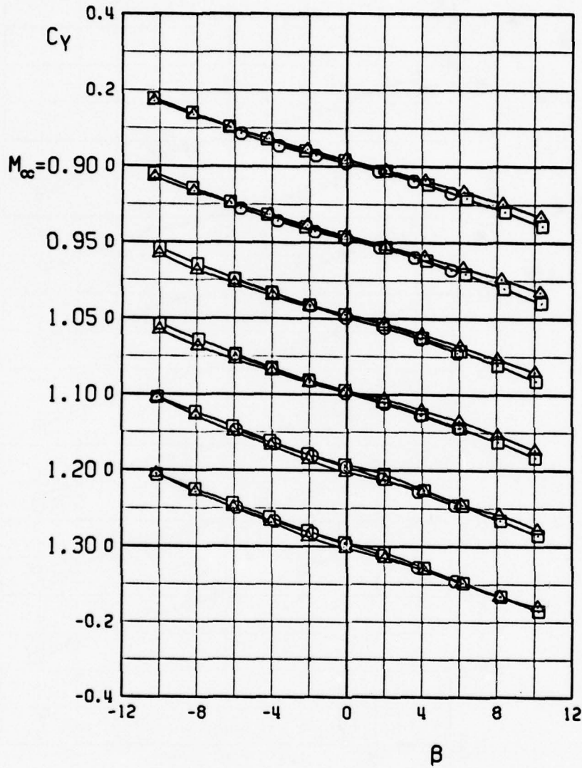
d. Concluded, \Lambda = 54 deg Figure 8. Continued.
