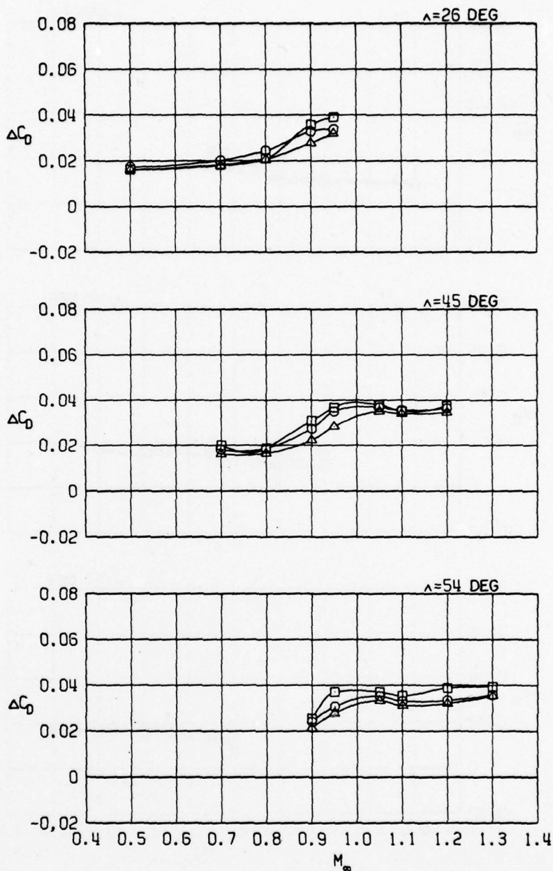
h. 12 SUU-30 stores (outboard pylons) Figure 15. Continued.
