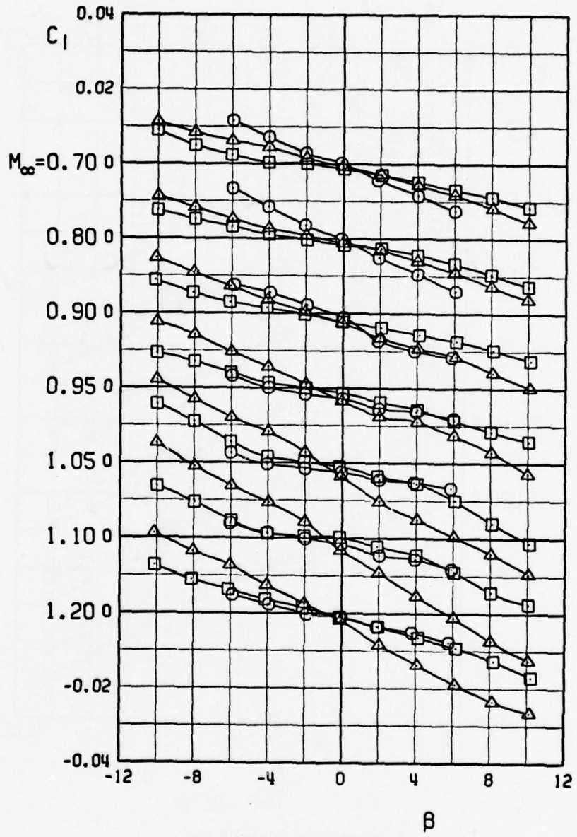
f. Continued, \Lambda = 45 deg Figure 8. Continued.
