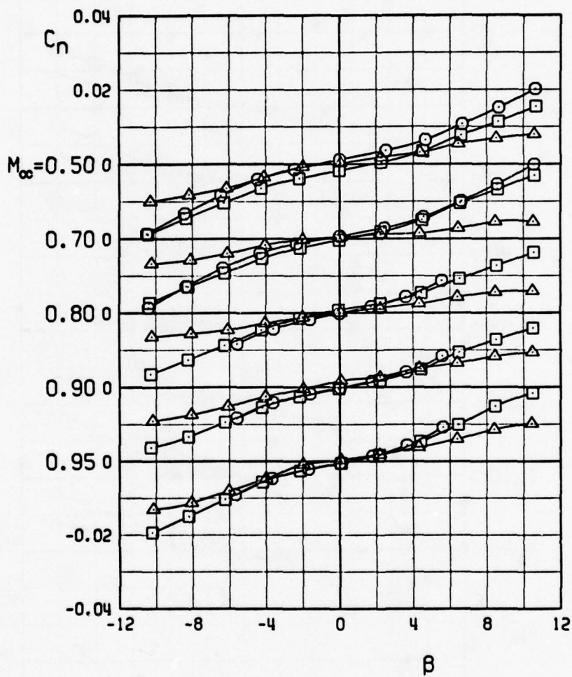
e. Yawing-moment coefficient, \Lambda = 26 deg Figure 8. Continued.
