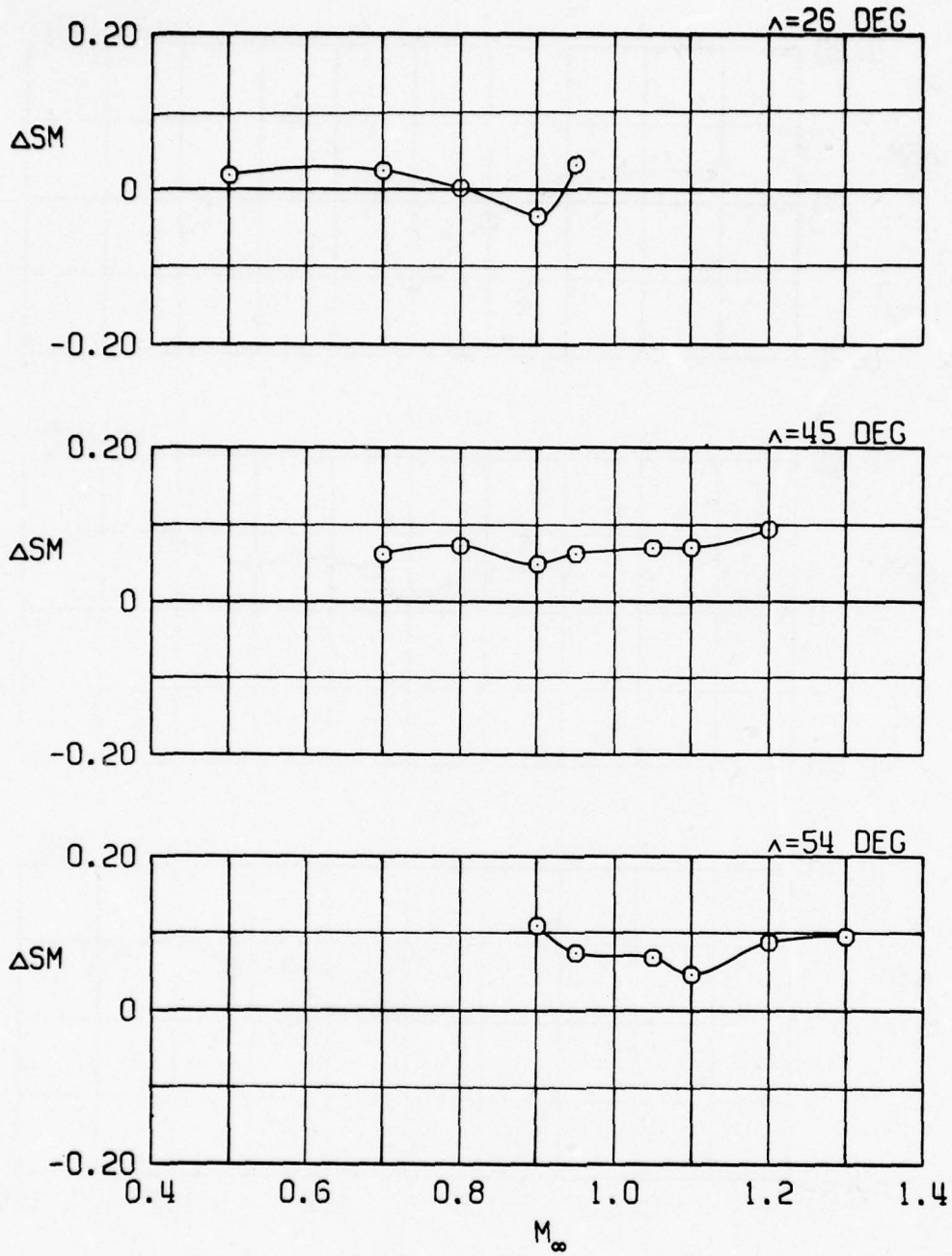
c. Four GBU-15CCW stores Figure 14. Continued.
