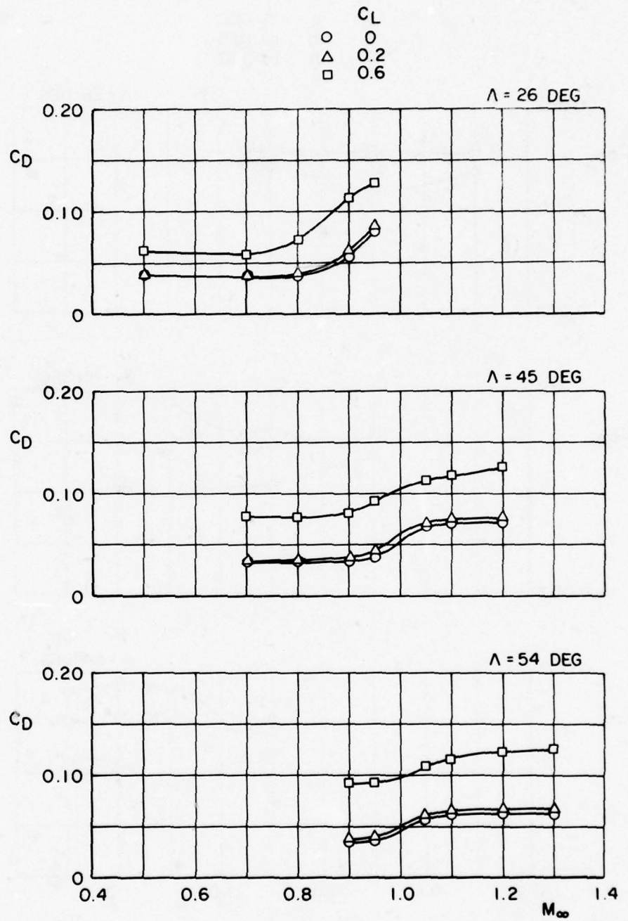
c. Drag coefficient Figure 9. Continued.
