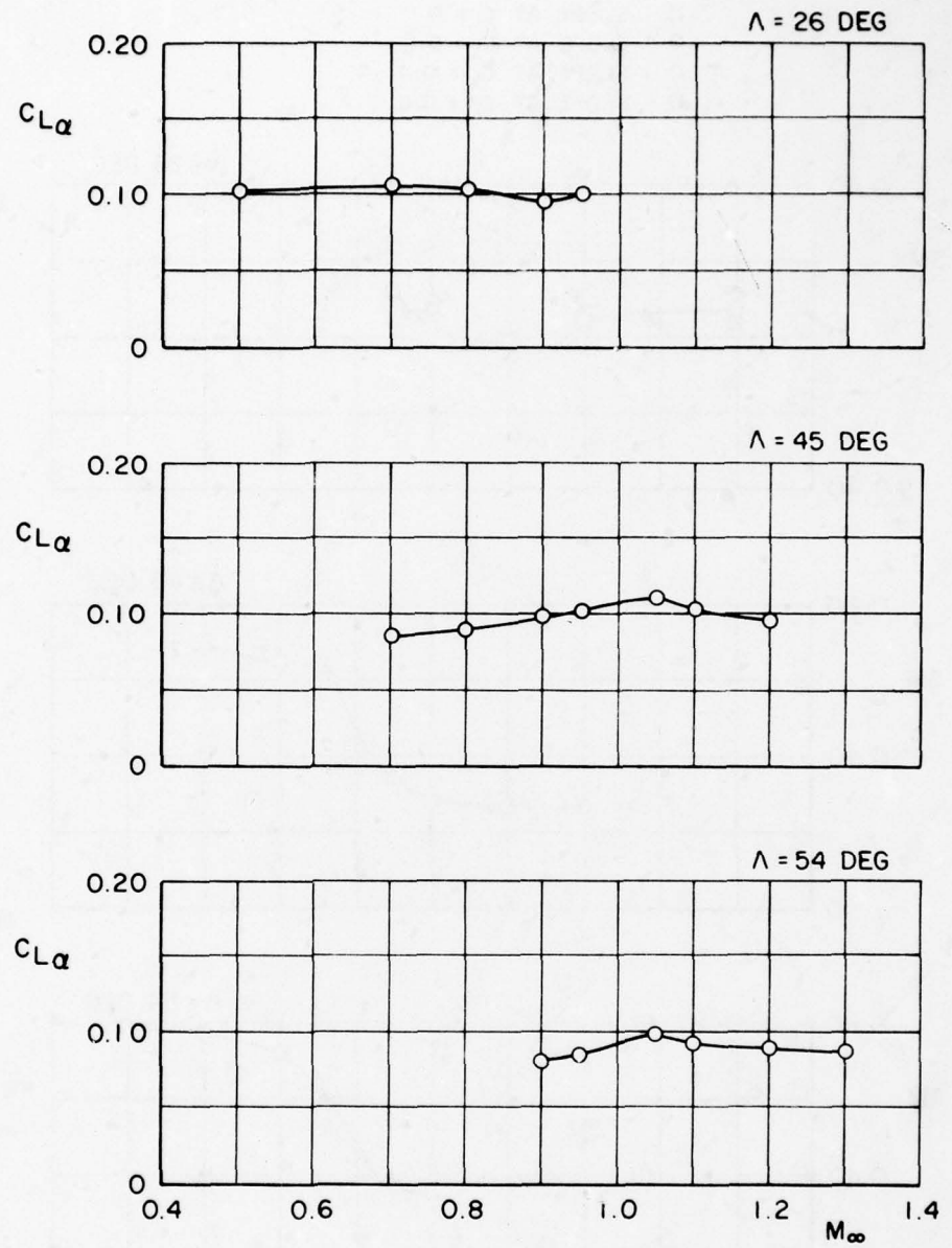
a. Lift curve slope
