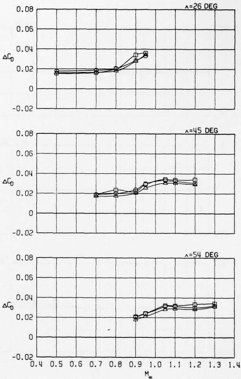
j. 22 MK-82SE stores Figure 15. Concluded.
