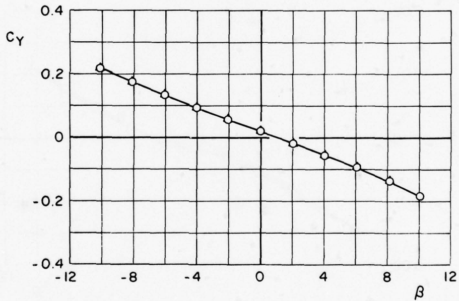
d. Side-force coefficient Figure 13. Continued.
