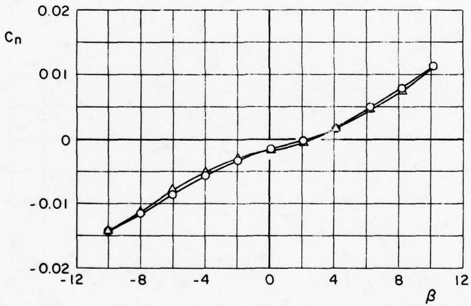
e. Yawing-moment coefficient Figure 13. Continued.
