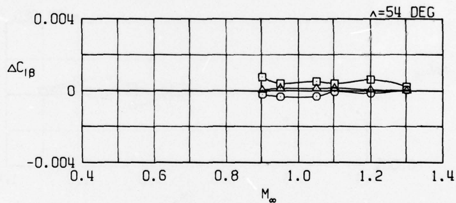
d. Four GBU-15CCW stores and extended Pave Tack pod Figure 17. Continued.
