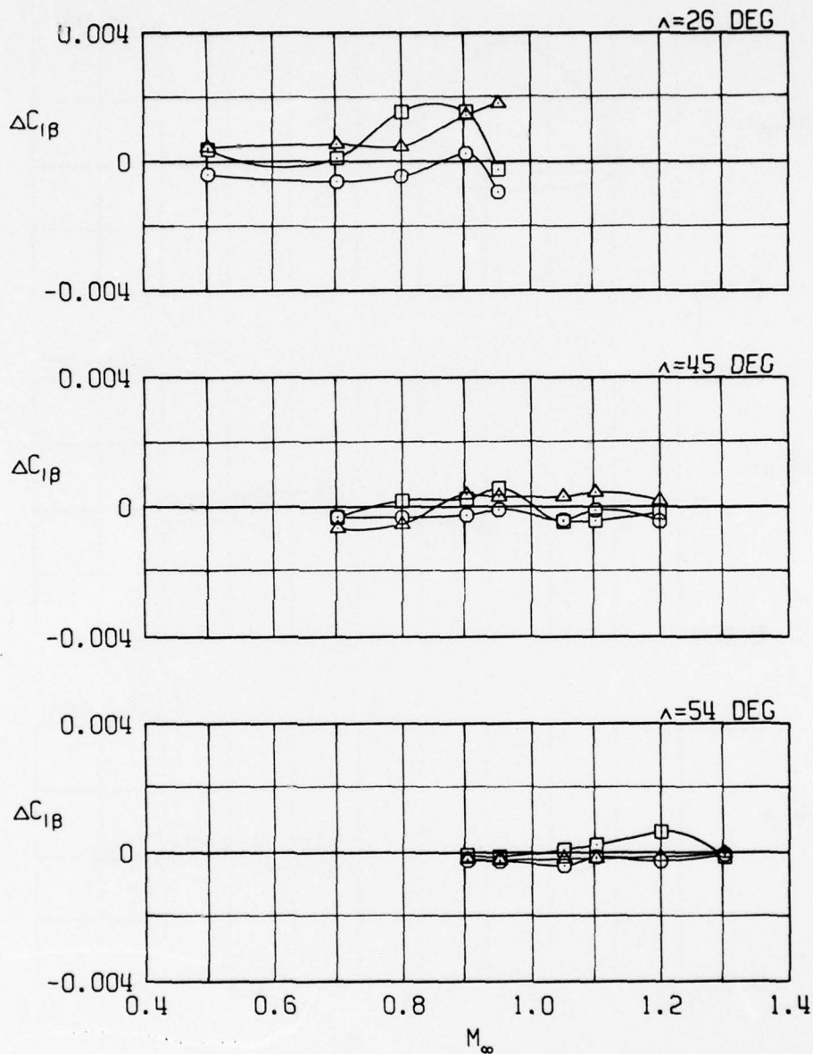
b. Four GBU-10 stores Figure 17. Continued.
