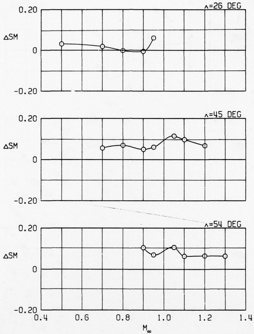
i. 12 MK-82SE stores (outboard pylons) Figure 14. Continued.
