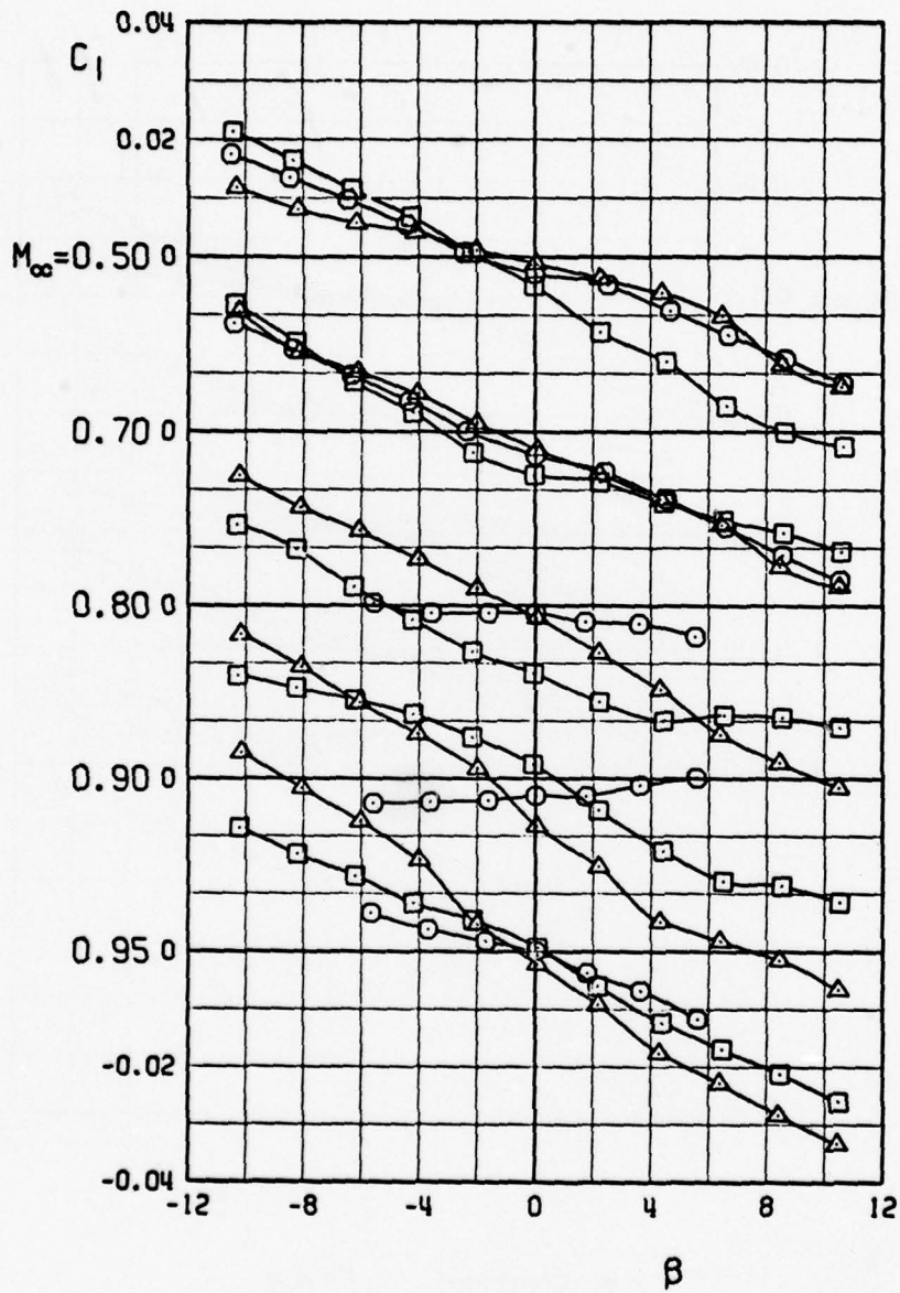
f. Rolling-moment coefficient, \Lambda = 26 deg Figure 8. Continued.
