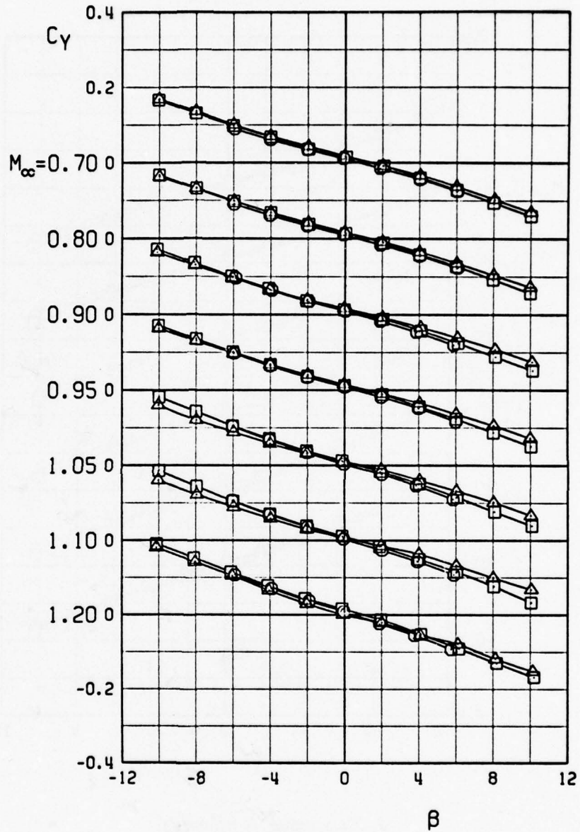
d. Continued, \Lambda = 45 deg Figure 8. Continued.
