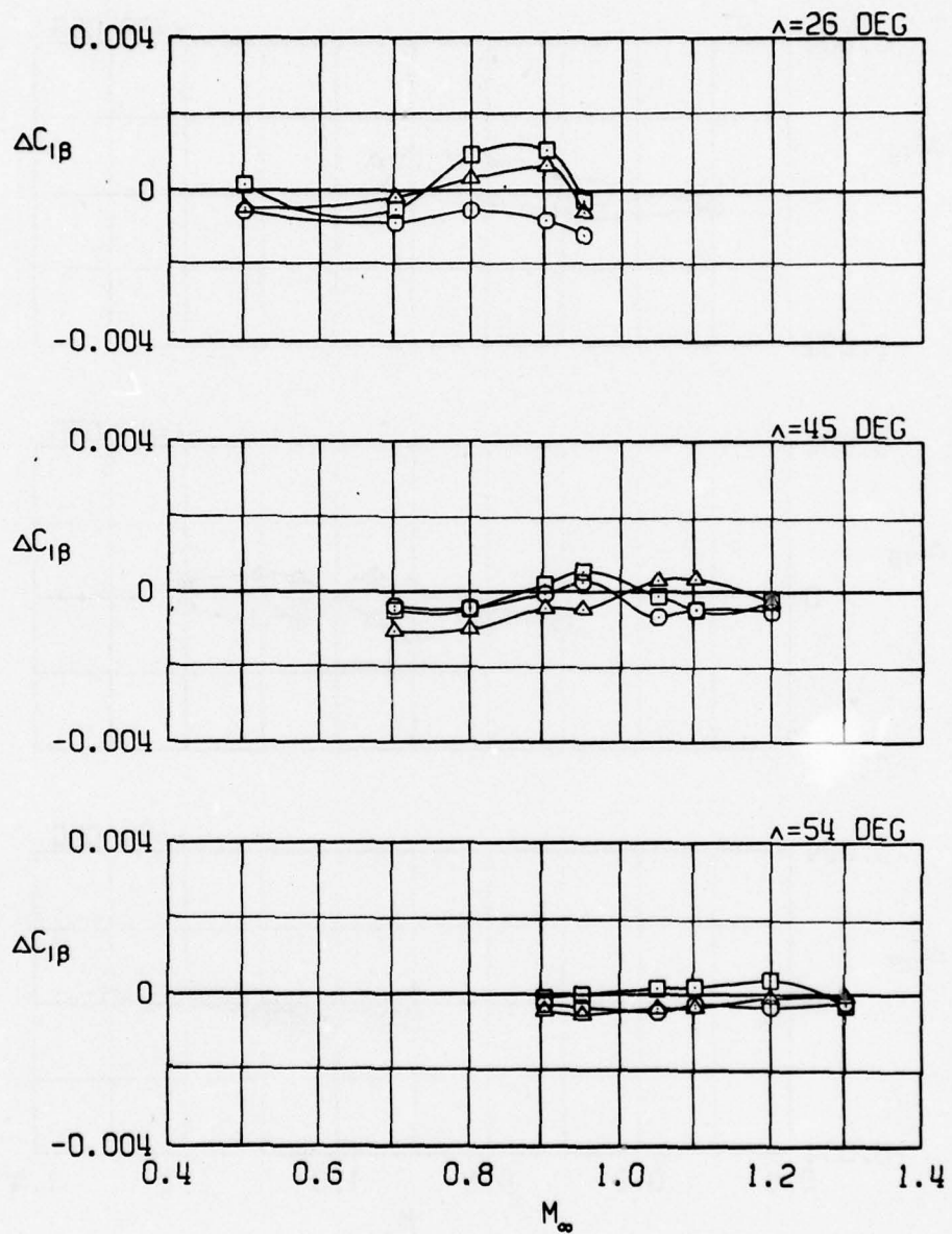
f. 16 Rockeye stores (slant 4 loading) Figure 17. Continued.
