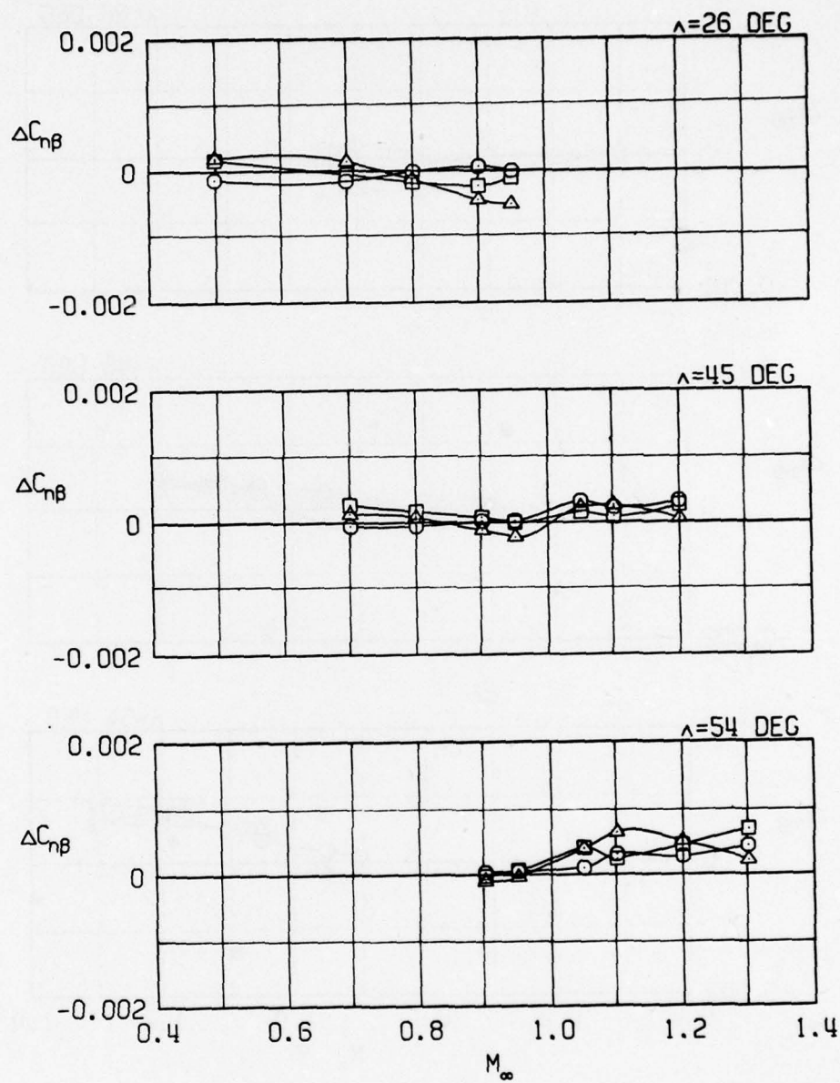
b. Four GBU-10 stores Figure 16. Continued.
