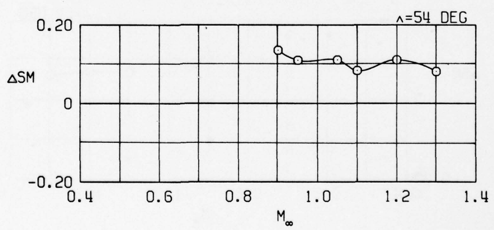
f. 16 Rockeye stores (slant 4 loading) Figure 14. Continued.
