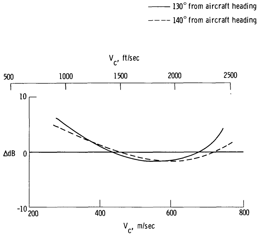
(a) Core jet velocity.
