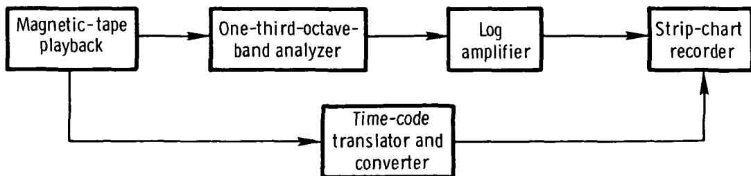
Figure 6. Block diagram of data reduction system.
