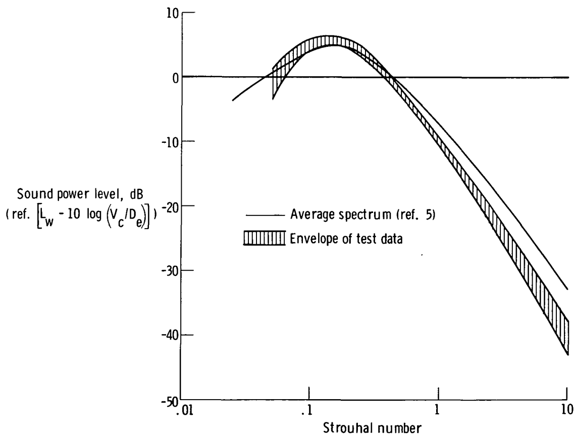
Figure 12. Normalized sound power spectra for one- and two-engine operation at three engine power settings.
